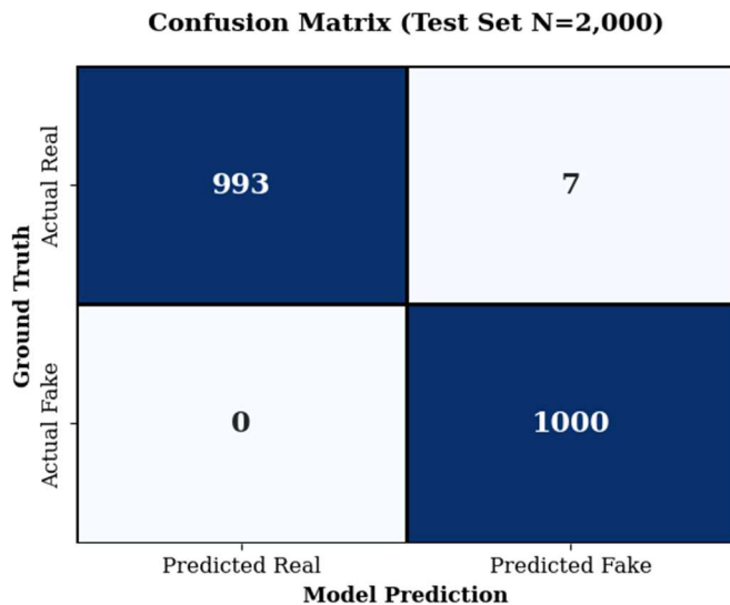
Figure 3: Confusion Matrix on the Test Set (2,000 images). The model achieves 100% recall on synthetic samples, successfully flagging all diffusion and GAN-generated instances with zero false negatives.
